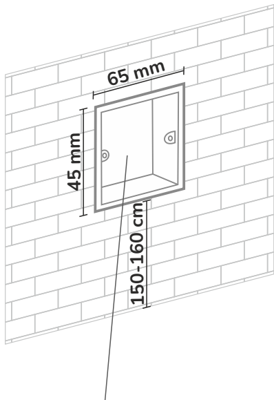
Mounting box
